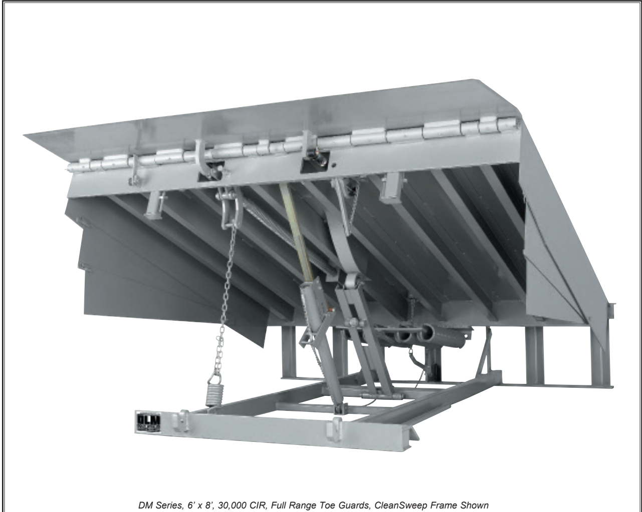
DM Series, 6' x 8', 30,000 CIR, Full Range Toe Guards, CleanSweep Frame Shown
